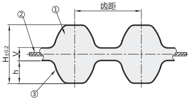
齿形：DS5M/DS8M/DS14M
