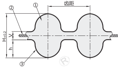
齿形：DH8M/DH14M
