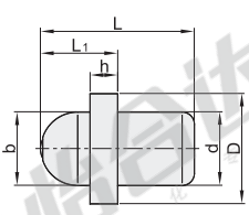
油嘴形状
