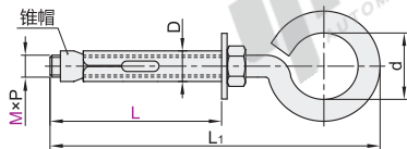
羊眼膨胀螺栓 TBF61/62
