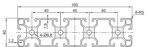
AOB05-40160
