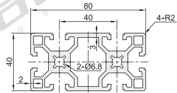
AOB03-4080E AOB05-4080E
