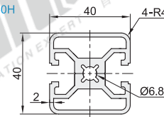
AOB05-4040T
