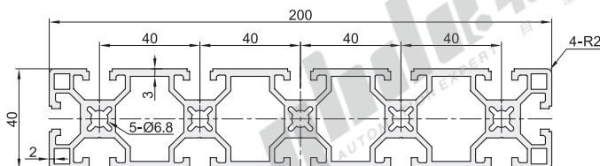
AOB05-40200E
