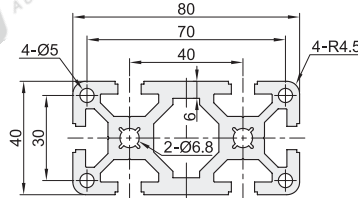
AOB03-4080J AOB05-4080J
