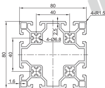
AOB05-8080F
