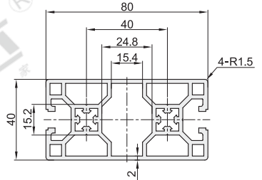
AOB05-4080H
