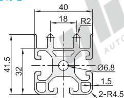
AMS05-OB40-E
