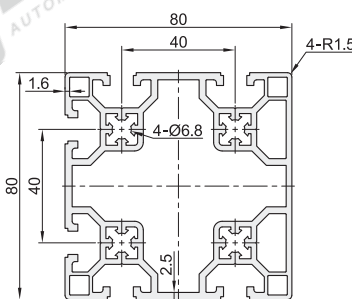
AOB05-8080FA
