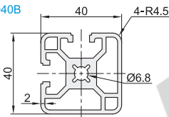
AOB05-4040H
