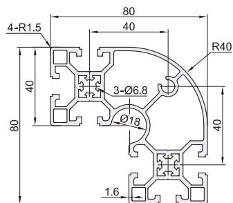
AOB05-8840RF
