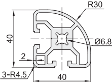
AOB05-4040R
