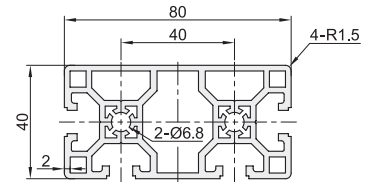
AOB05-4080H
