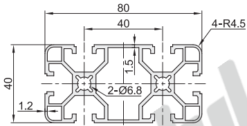
AOB05-4080C
