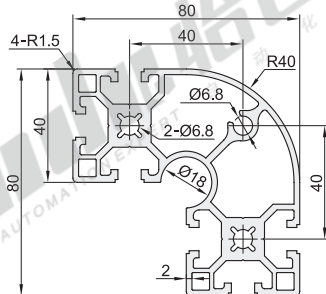
AOB05-8840RE
