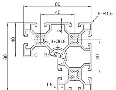
AOB05-8840
