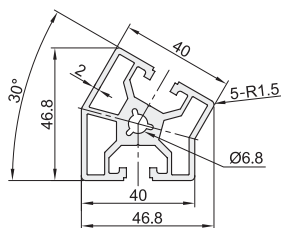
AMS05-OB40-E
