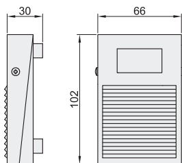
单脚踏 ZHB93
