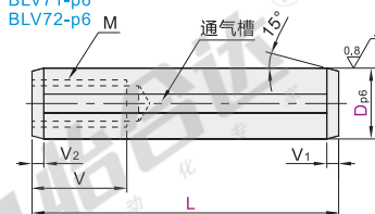
带通气槽型·公差 +0.010 / +0.005
