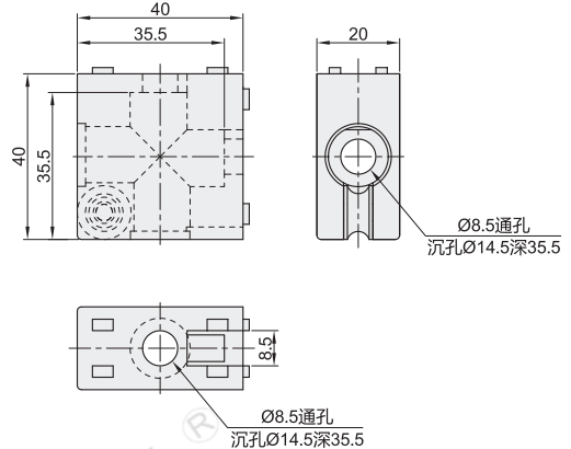
滑动固定块 AMS07-C
