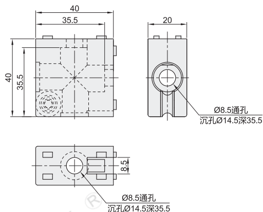
滑动固定块 AMS07-C
