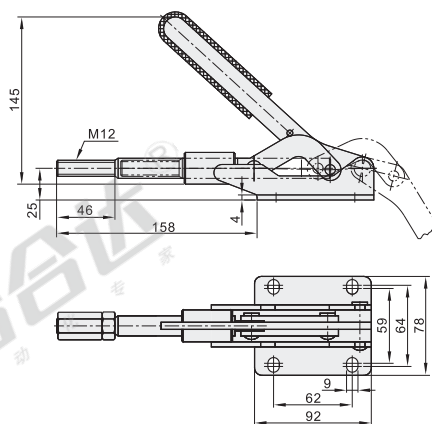
WDC303-EM
