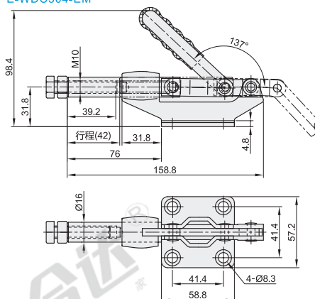
WDC304-EM E-WDC304-EM
