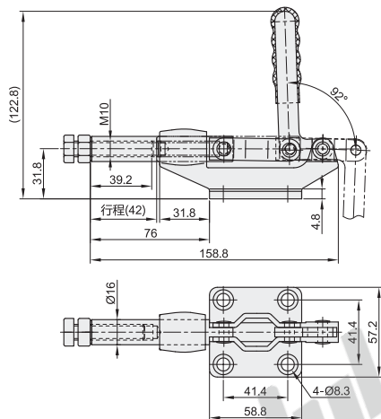
WDC305-EM
