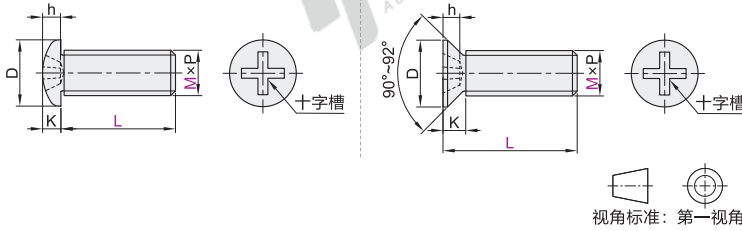
十字槽盘头螺钉 PACK-TBD01/02/03/04
