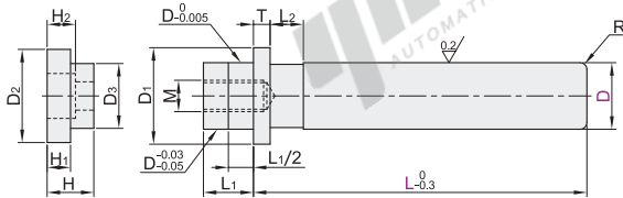
装卸型·无挡块 OFJ01
