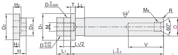
装卸型·可动挡块 OFJ02
