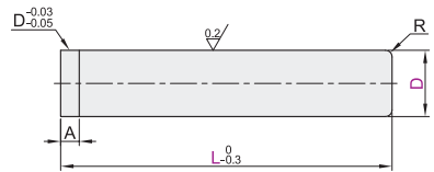
压入型·无挡块 OFJ11
