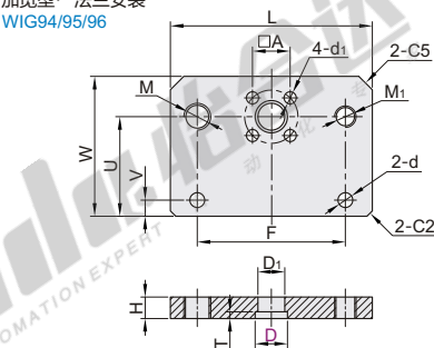
加宽型·法兰安装 WIG94/95/96
