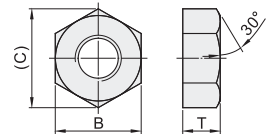
附件螺帽
