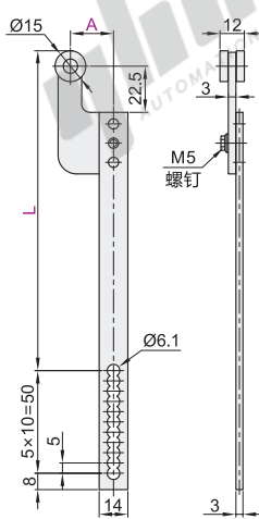
带圆眼多孔连杆 XAV56
