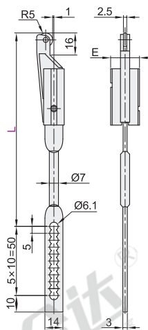
带滚轮连杆 XAV61/62
