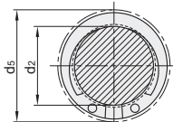
挡圈装配尺寸
