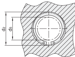
挡圈装配尺寸
