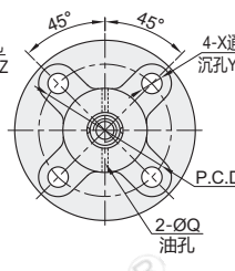
D=8/16/20 (2列滚珠)
