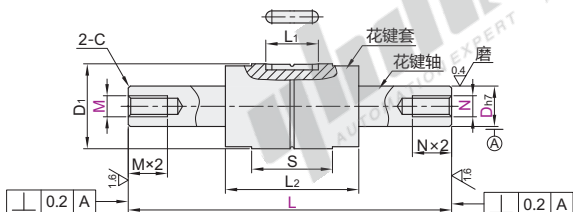
D ≤ 20 (2列滚珠)
