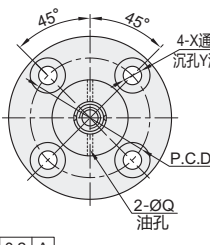
D=6/10/13 (2列滚珠)
