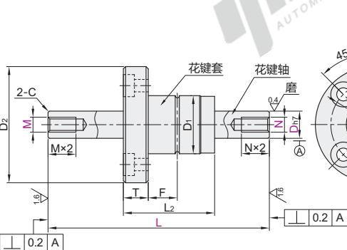
D=6/10/13 (2列滚珠)
