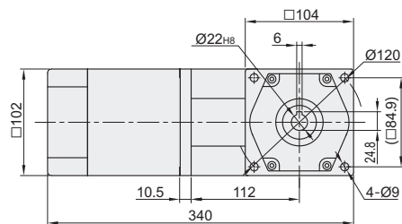
减速机+电机 (输出轴:空心轴) (ZKR88+ZKR16)
