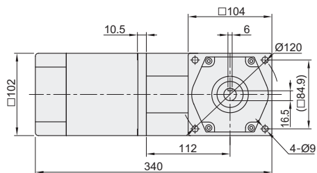
减速机+电机 (输出轴:实心轴) (ZKR88+ZKR15)
