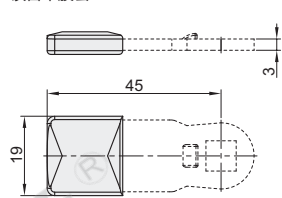
锁舌带胶套
