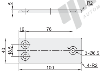
AGT50-A-40100
