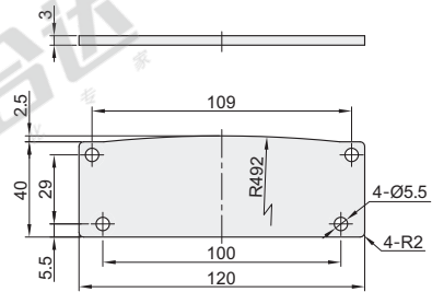
AGT50-S-40120
