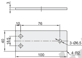
AGT50-S-40100
